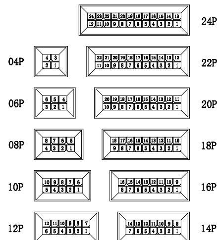
CIRCUIT SIZE LAYOUT
